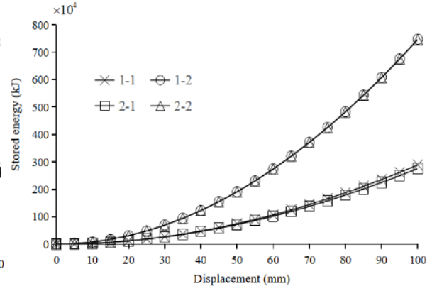
Fig. 18. Displacement-stored energy
