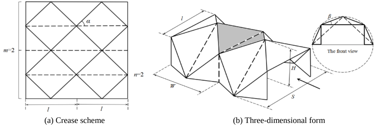
Fig. 7. Target structure
