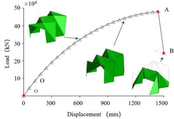
(b) Triangle enhancement scheme
