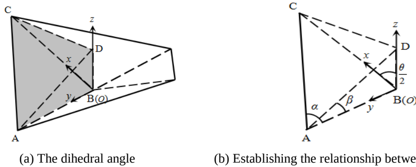
Fig. 8. Analysis of the relationship between plane angle \alpha and dihedral angle \theta
